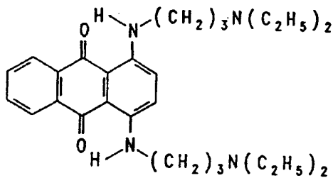
Compound 1b
